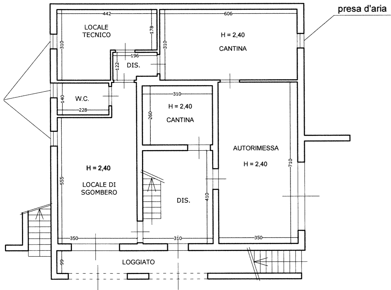
PIANO SEMINTERRATO
